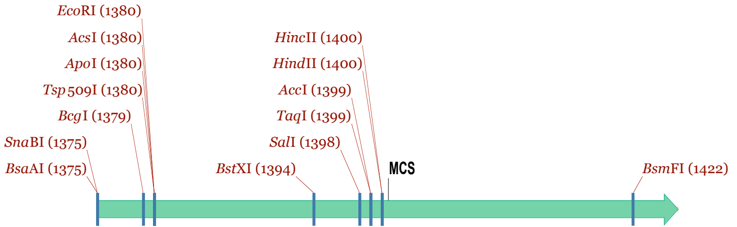
Fragment of pBABEhygro 51 bp (molecule 5558 bp)
