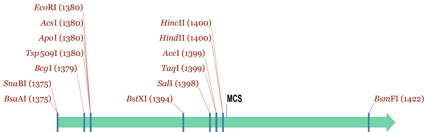
Fragment of pBABE 51 bp (molecule 4508 bp)
