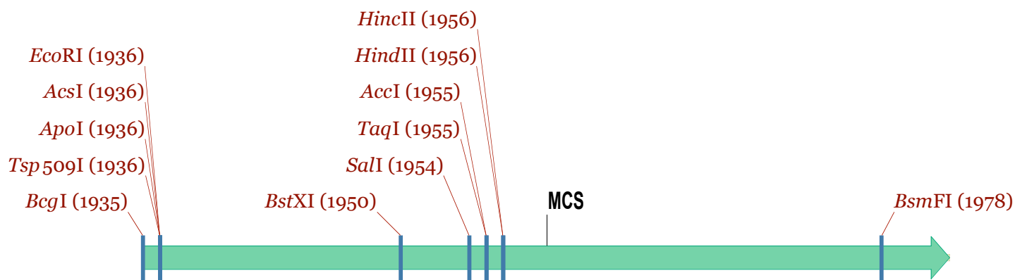
Fragment of pBABE HRas puro 47 bp (molecule 5725 bp)
